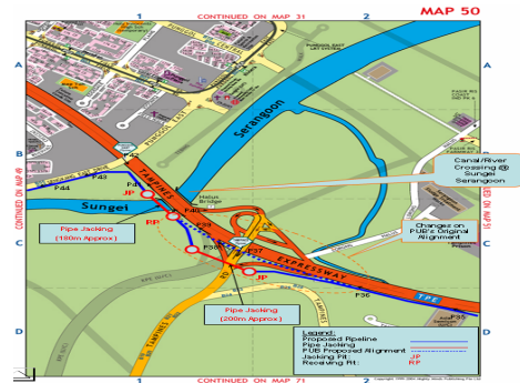
Location Plan of NEWater Pipeline
