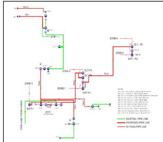
Schematic layout of proposed Water Supply System
