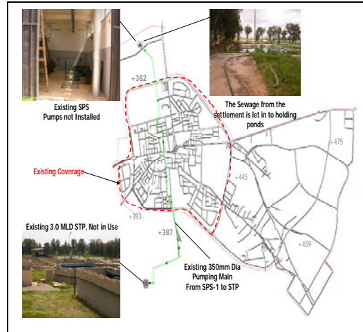
Existing Sewerage System
