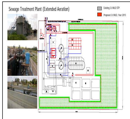
Sewage Treatment Plant
