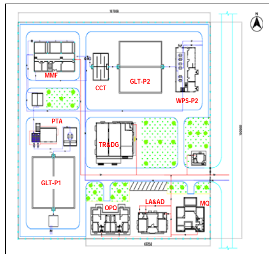
Water Treatment Plant: Layout
